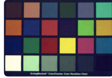
JPEG 75% quality
