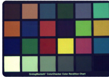
JPEG 100% quality
